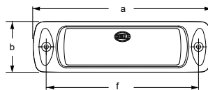
Sea Hawk R Recessed Mount
